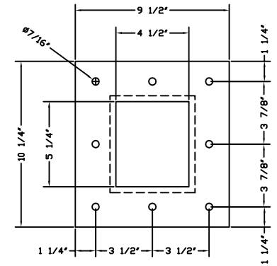
DISCHARGE FLANGE DETAILS
