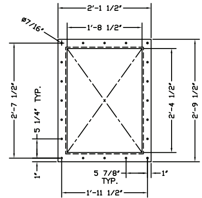
DISCHARGE FLANGE DETAILS
