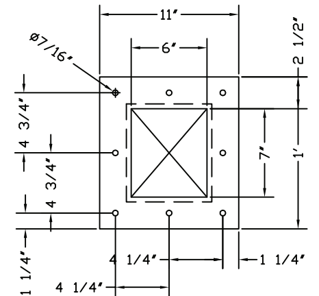
DISCHARGE FLANGE DETAILS
